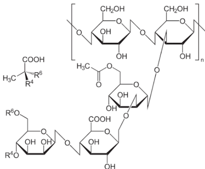
Figure 3 – the structure of xanthan
