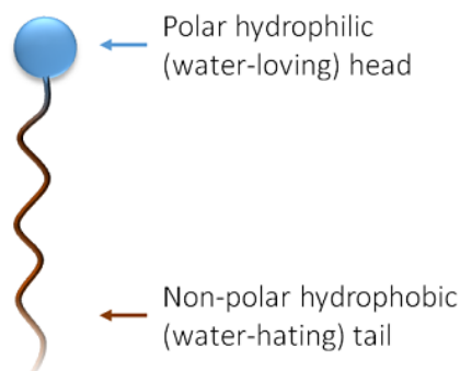
Figure 4 – the general structure of a surfactant
