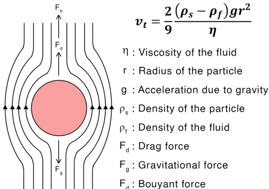
Figure 2 – Stokes' Law and what each variable means
